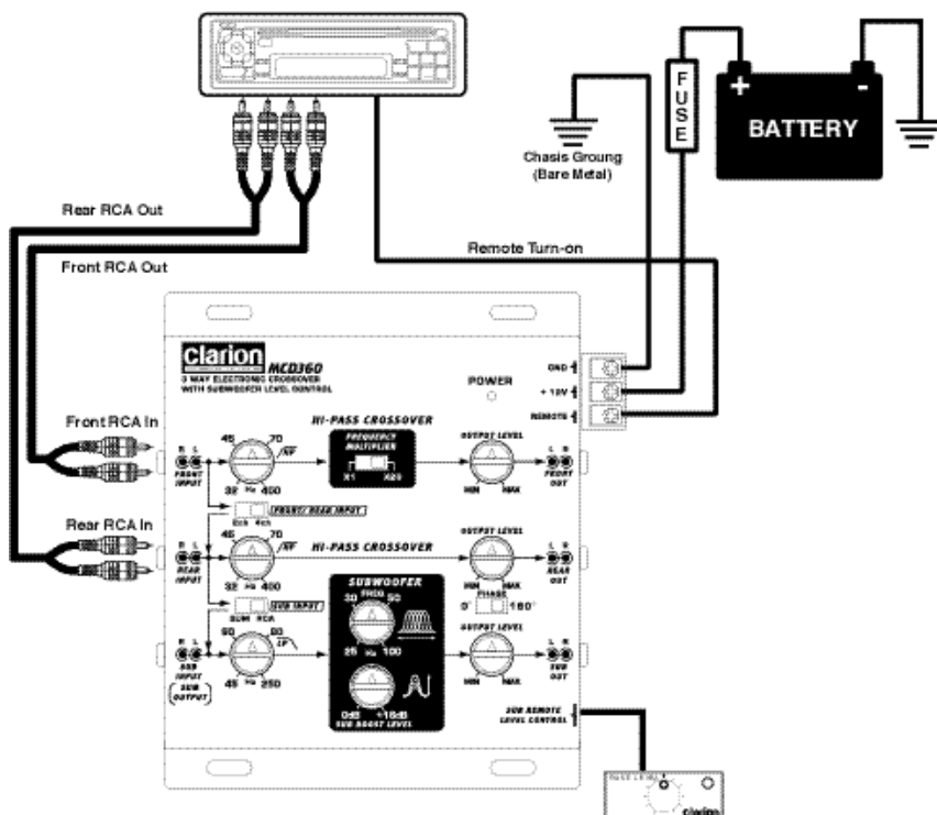
Figure 3 - Electrical connections for the MCD-360
