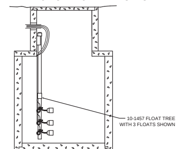
TYPICAL FLOAT HANGER ON CONCRETE PITS OR SEPTIC TANK RISERS
