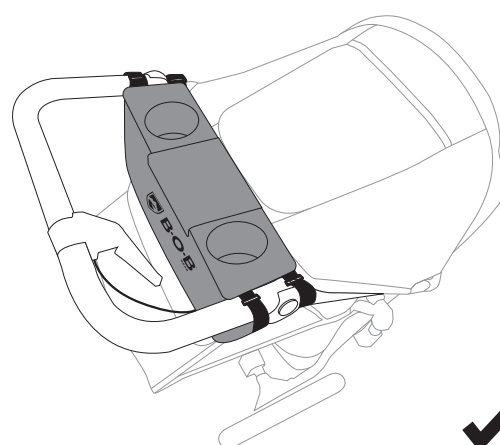
Handlebar Console Installed on Stroller.
