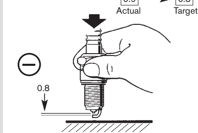
Narrowing the electrode gap Values in mm
