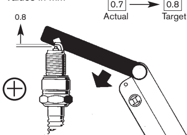
Widening the electrode gap Values in mm
