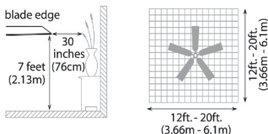
downrod installation
