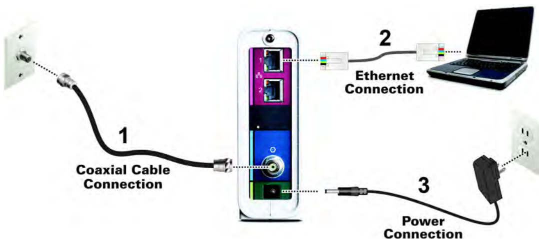
SB8200 connection diagram
