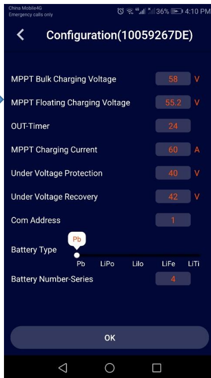
11. Setting for lead acid battery
