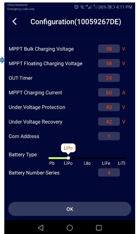
12. Setting for lithium battery
