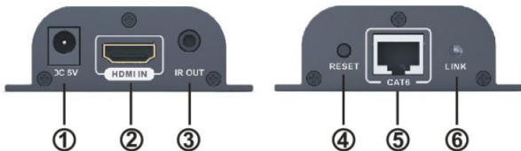
Figure 1: Transmitter (TX)
