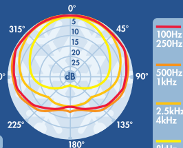
Polar Response
