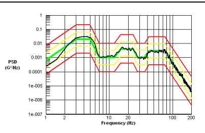
Block 12 Face 4 Test Vibration Profile
