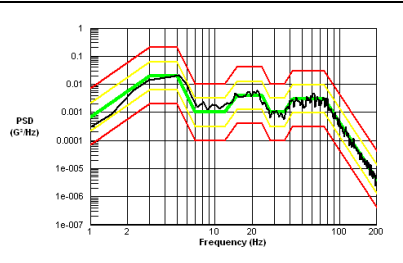
Block 12 Face 3 Test Vibration Profile
