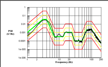
Block 12 Face 3 Test Vibration Profile
