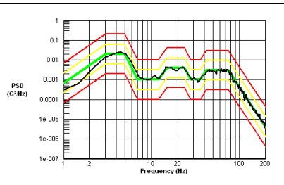
Block 12 Face 6 Test Vibration Profile
