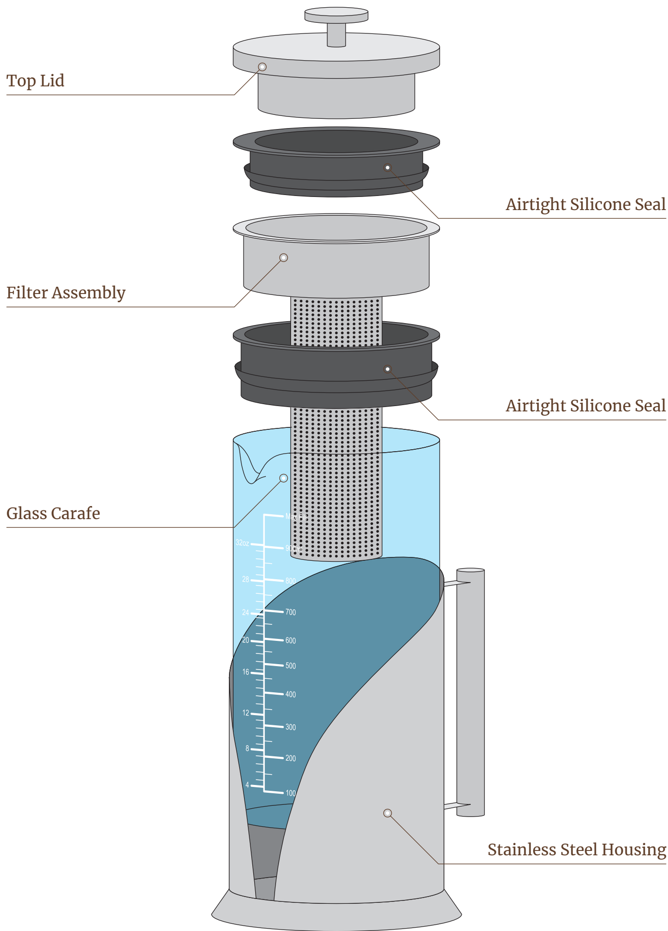
Fig 1. Exploded Diagram
