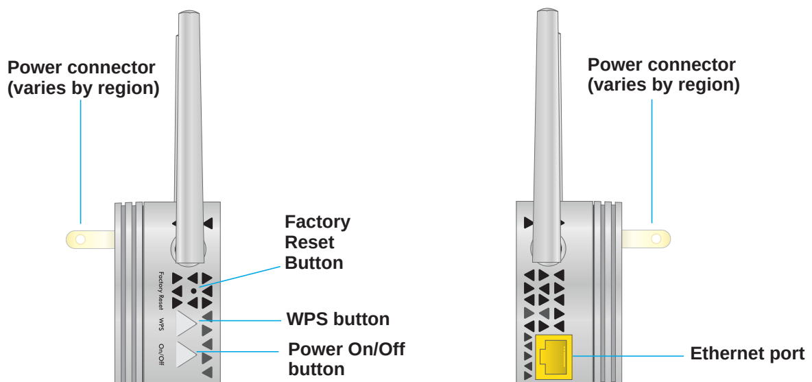
Figure 2. Buttons and port on the side panels
