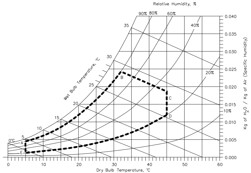
Figure 8-3 Internal drive: Operating tape path temperature and humidity ranges
