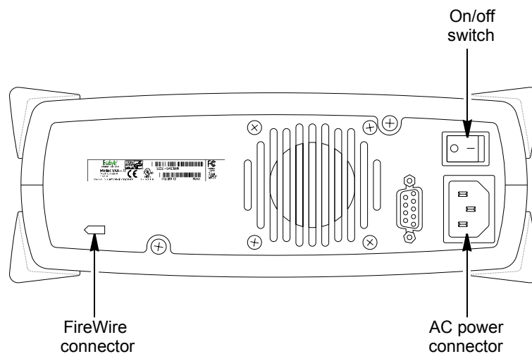
Figure 2-9 External FireWire drive: back-panel components
