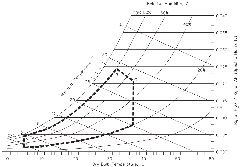
Figure 8-4 External drive: Operating tape path temperature and humidity ranges
