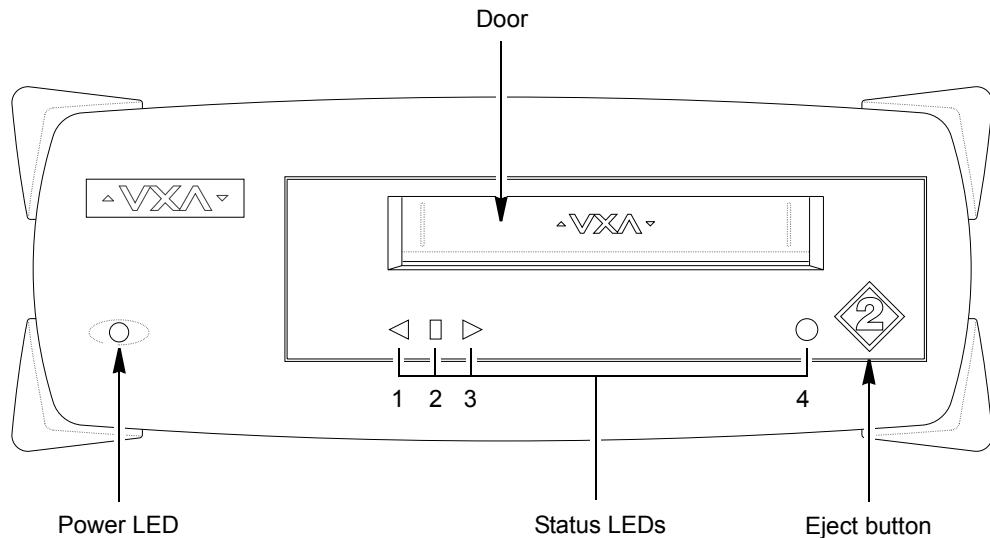
Figure 1-3 External drive: front-panel components
