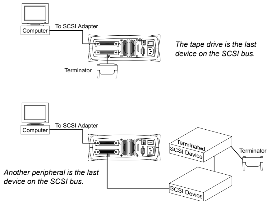
Figure 2-8 Terminating the SCSI bus for the external model
