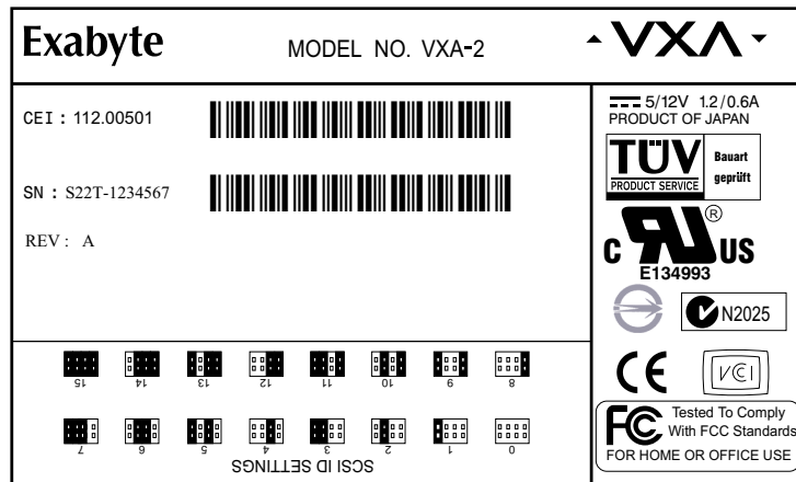
Figure 1-8 Top-panel label (SCSI tape drive)
