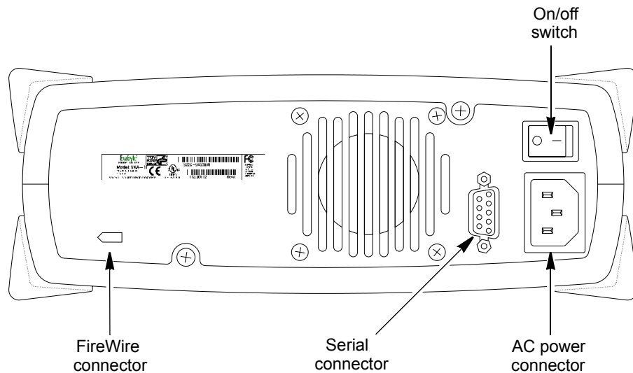
Figure 1-6 External FireWire drive: back-panel components
