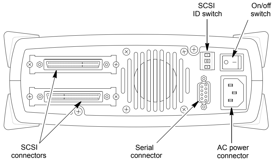
Figure 1-5 External SCSI drive: back-panel components
