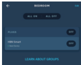
Alexa App
