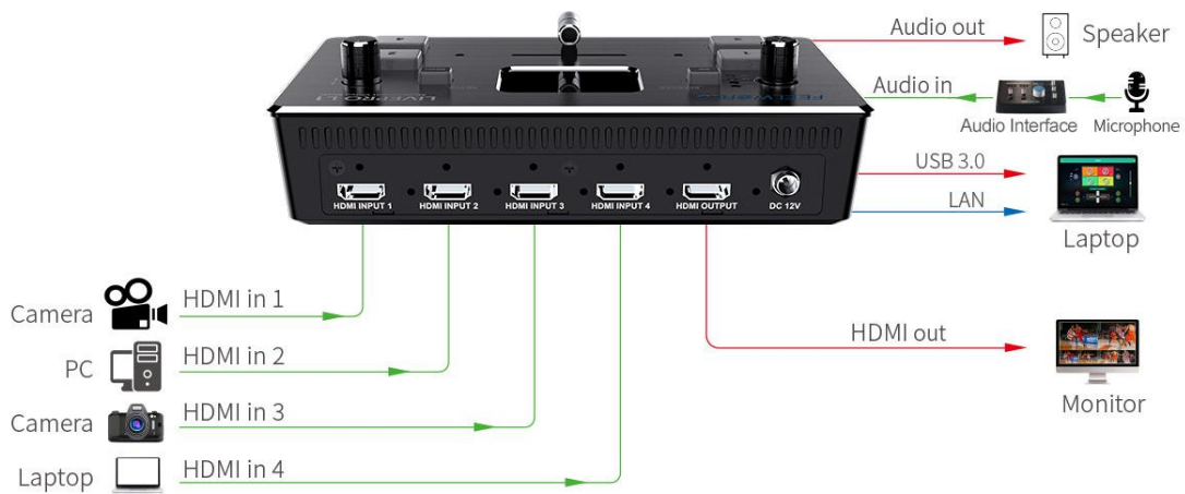
LIVEPRO L1 System Connection Diagram
