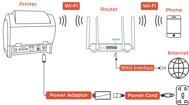
Wi-Fi Connection
