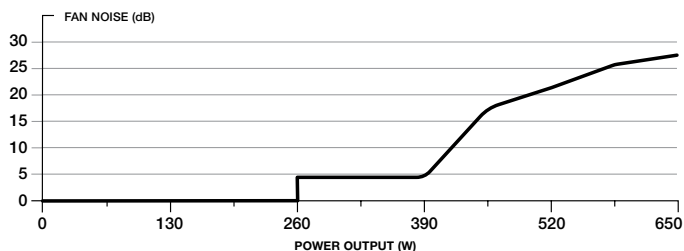
CORSAIR RM650x POWER SUPPLY FAN NOISE CURVE
