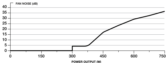
CORSAIR RM750x POWER SUPPLY FAN NOISE CURVE
