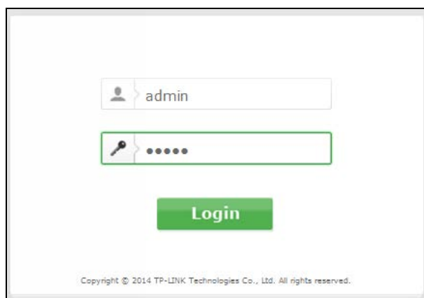
Figure 3-4 Login Windows
