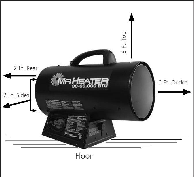
Figure 2 Clearance Diagram
