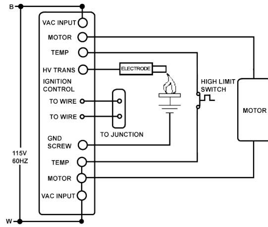
SCHEMATIC DIAGRAM
