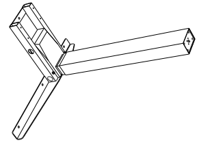
Step 2 Assembly
