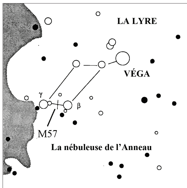
Fig. 17 Ring Nebula
