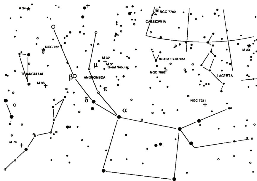
Fig. 16 Galassia Andromeda
