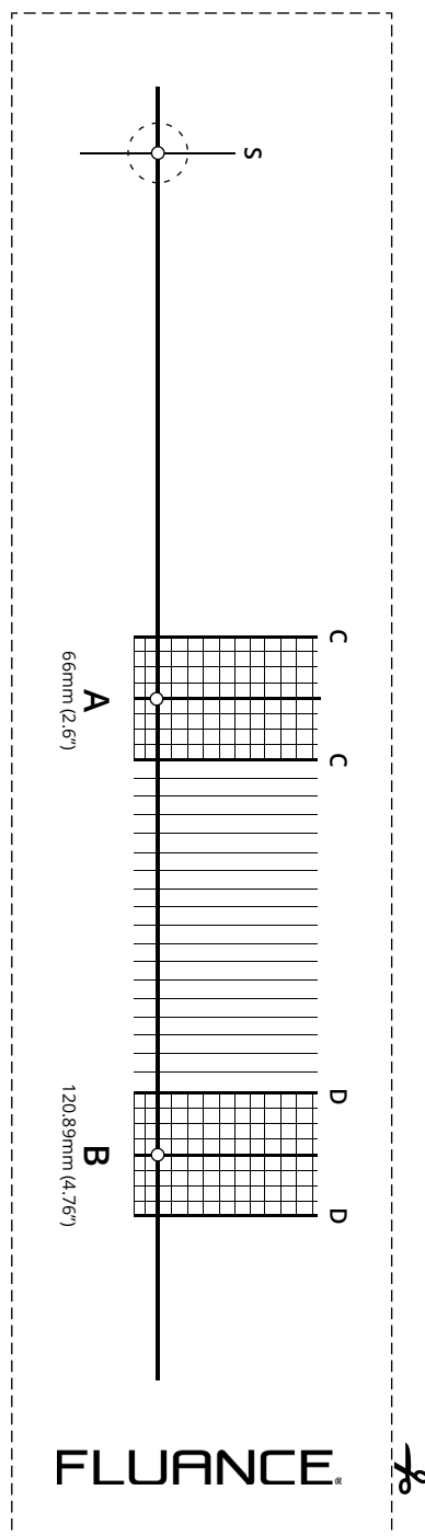
Cartridge Alignment Protractor Cutout
