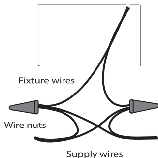
WIRING DIAGRAM
