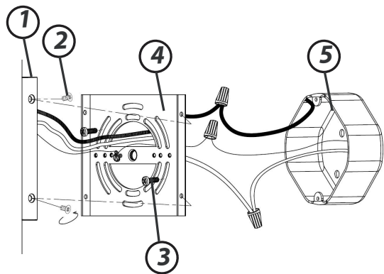
DRAWING 2 - ASSEMBLY
