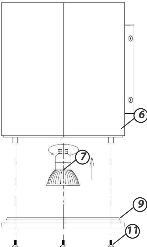
DRAWING 2 - ASSEMBLY
