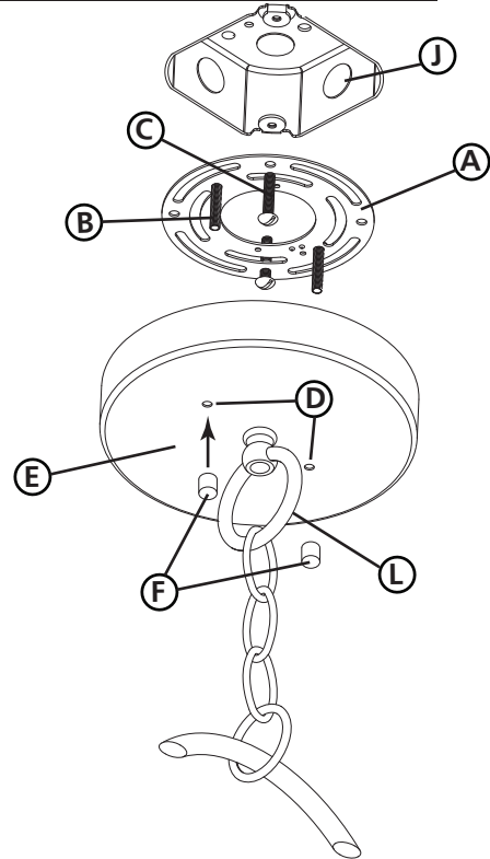
DRAWING 2 - ASSEMBLY
