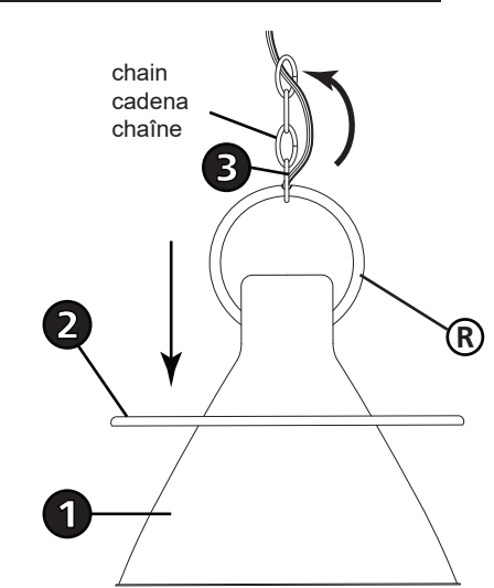
DRAWING 2 - ASSEMBLY
