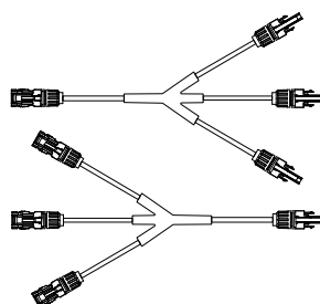
MC4 Solar Charging Connector
