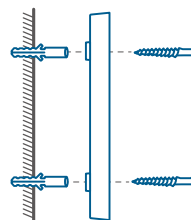
Mounting Bracket
