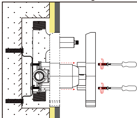
Before tiling
