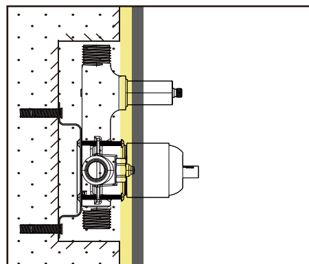
Finished Wall
