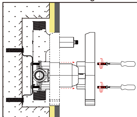
Before tiling
