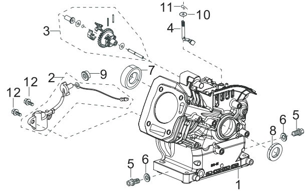
Fig. 2 - Crankcase Assembly
