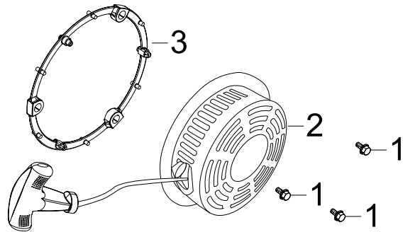
Fig. 7 - Recoil Starter
