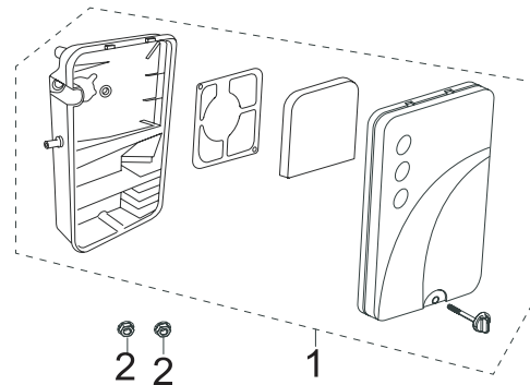
Fig. 10 - Air Cleaner
