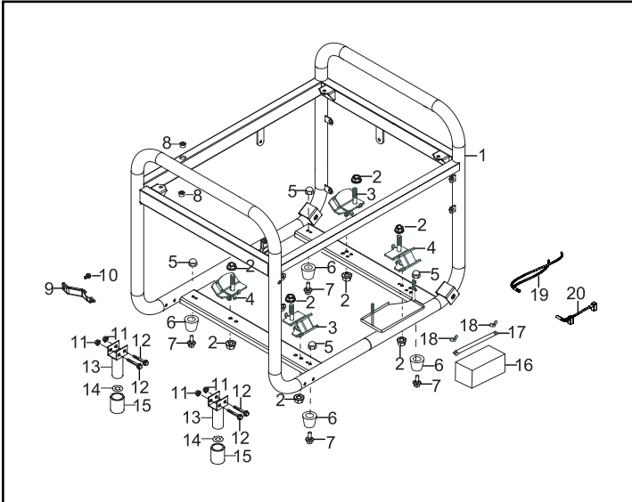
Fig. 16 - Frame, Engine
