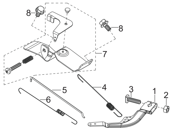
Fig. 12 - Control Assembly
