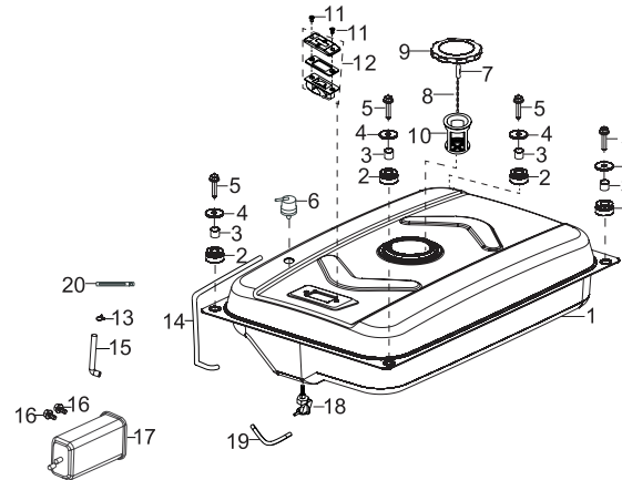
Fig. 15 - Tank, Fuel
