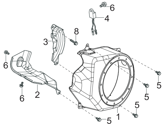
Fig. 8 - Shroud
