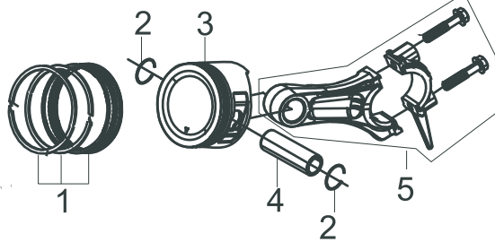
Fig. 5 - Piston Ring / Connecting Rod
