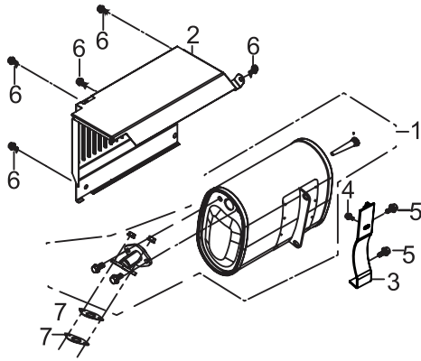
Fig. 14 - Muffler Assembly
