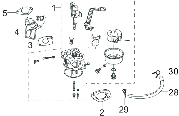
Fig. 9 - Carburetor Assembly
