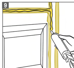
9 Apply additional layers of Paste over previous layers of Paste and Tape.
