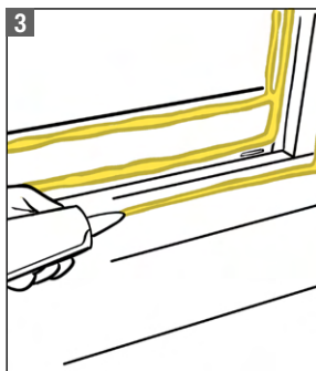
3 Apply Paste to window seams.
