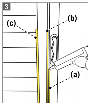
Apply an even coat of Paste where indicated above.
