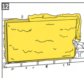
12 Brush an overlapping coat of Liquid on top of Paste and where it meets wall.
