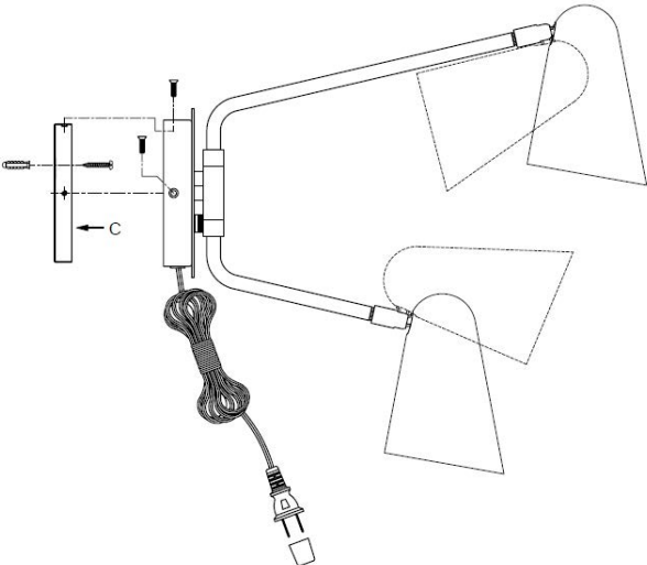
Drawing 3- Fixture diagram
