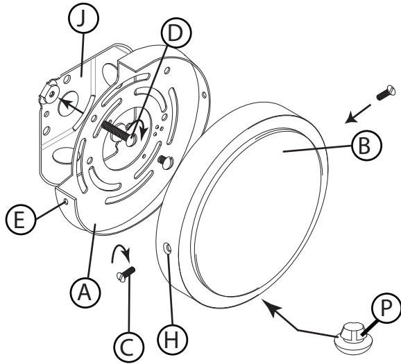
Drawing 2- Fixture diagram
