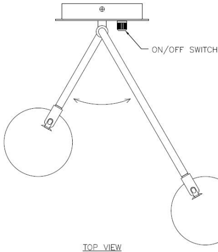
Drawing 3- Fixture diagram
