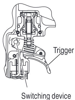
Enlarged view of the valve part
