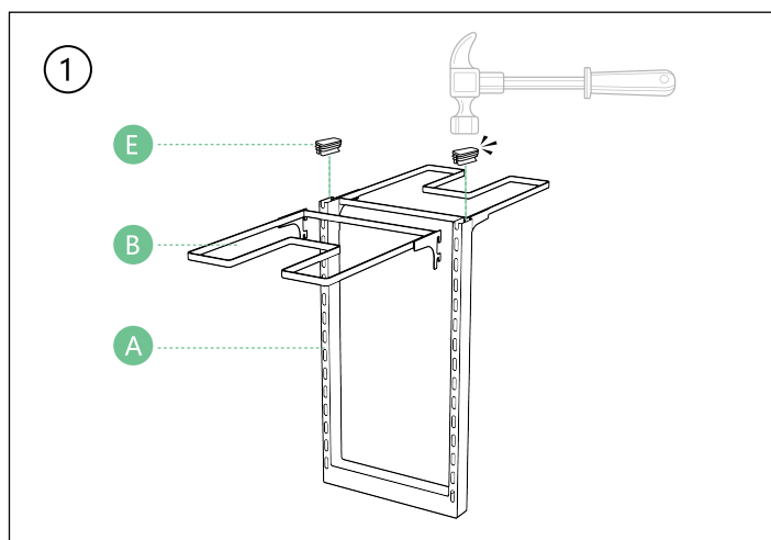
Install the base support rack
