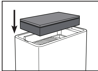
d. Insert Combination Filter into the unit with the HEPA portion facing into the unit. Consult the arrow on the filter for correct installation direction.
