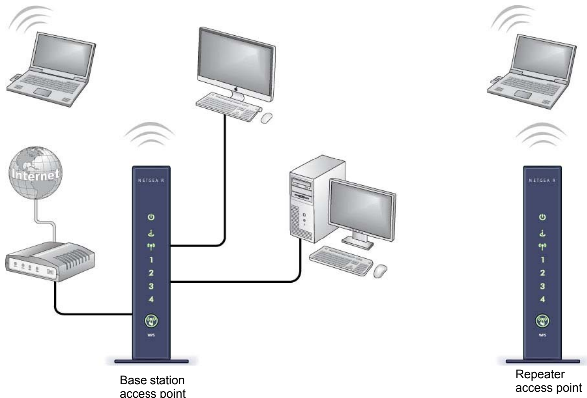
Figure 8. Wireless repeating scenario
