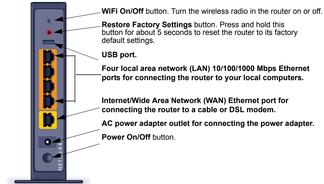
Figure 3. Back panel
