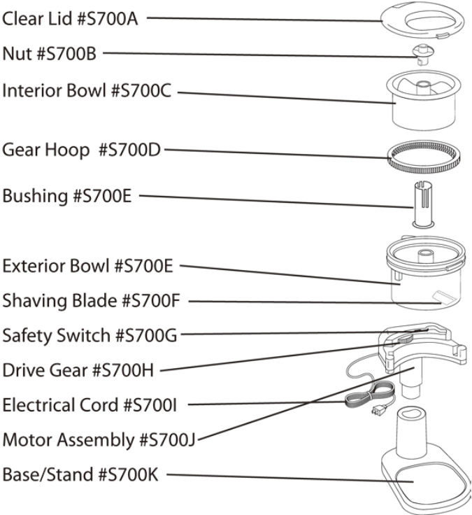
Figure A. Assembly/Parts Diagram for S700
