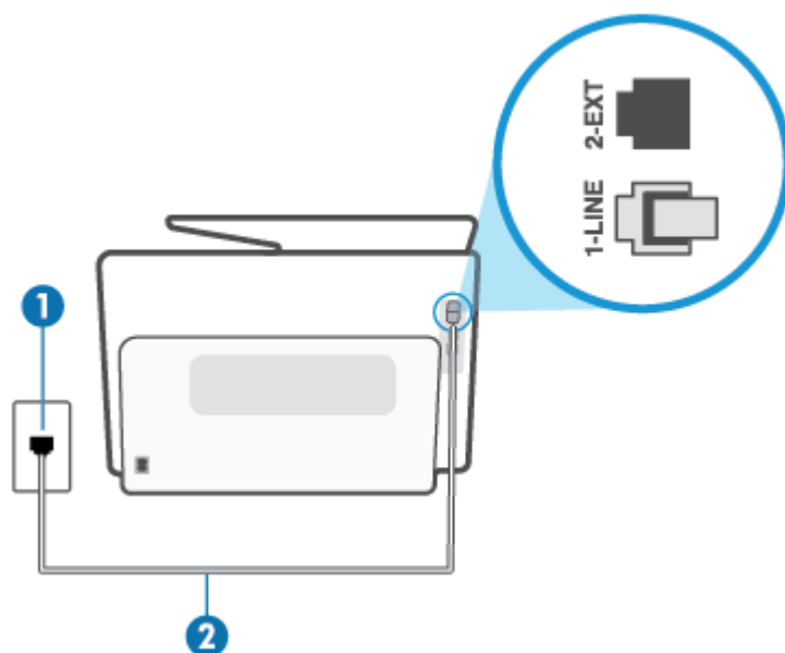
Figure 11-1 Back view of the printer
