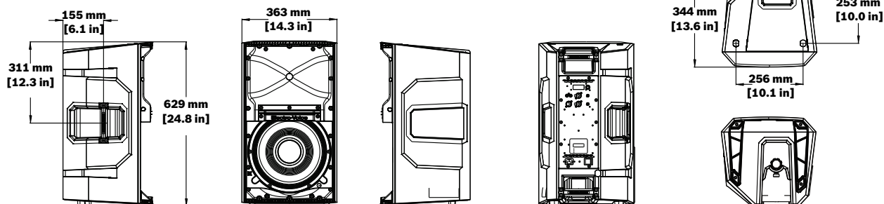
Figure 9.2: ELX200-12P dimensions
