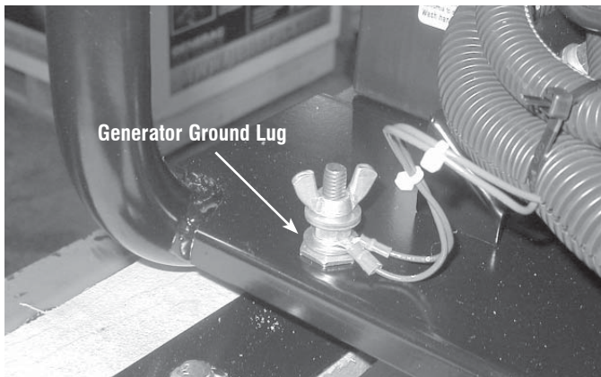
Figure 15 - Grounding the Generator
