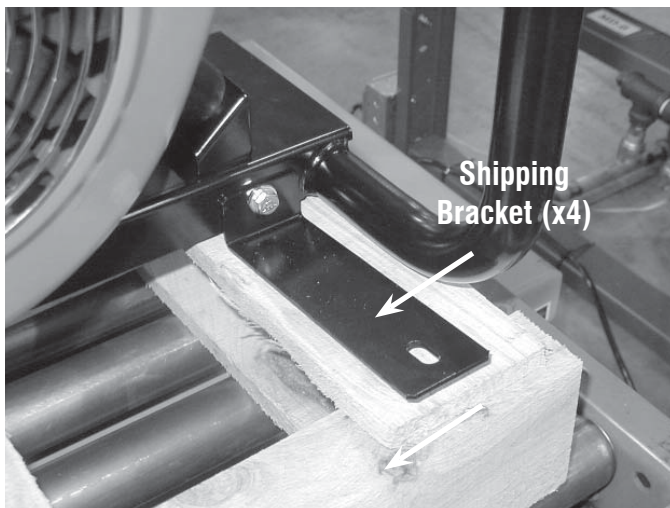
Figure 1 - Bracket Removal
