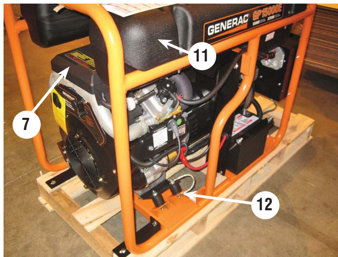
Figure 5 - Generator Controls
