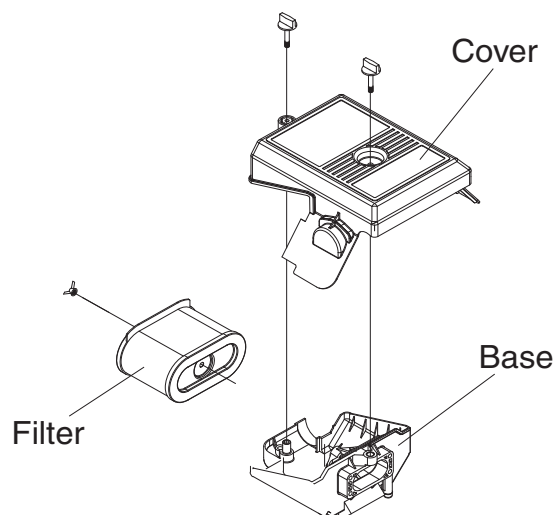
Figure 21 - Air Cleaner
