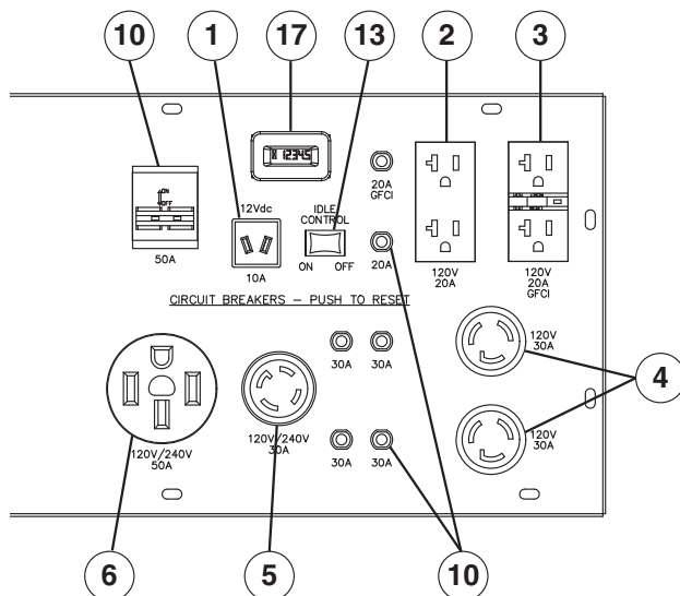
Figure 4 - Control Panel
