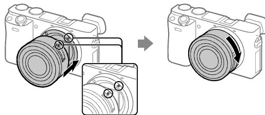
Mounting indexes
