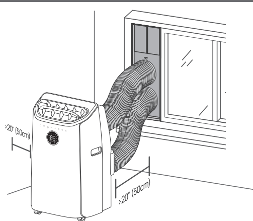
Sliding Window
