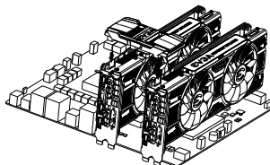
2-way SLI: Install your second GeForce graphics card in to the secondary PCI Express x16 slot. Connect the two cards together using the 2-way/new 2-way SLI bridge connector that came with your SLI-ready motherboard.
