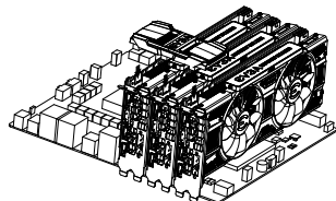
3-way SLI: Install the third GeForce card into the tertiary PCI Express slot on the motherboard. Connect the GeForce cards together using the 3-way SLI bridge connector that came with your SLI-ready motherboard.
